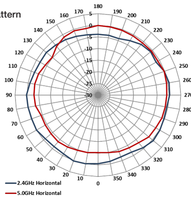
E-Plane Pattern
